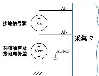
图 4-5-5 接地信号源的差分 (DIFF) 连接
